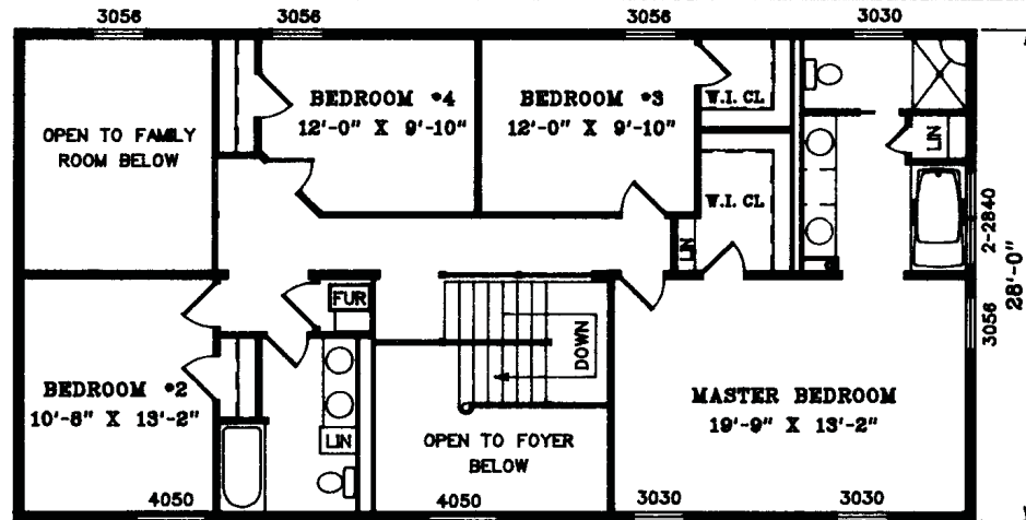
2ND STORY FLOOR PLAN
