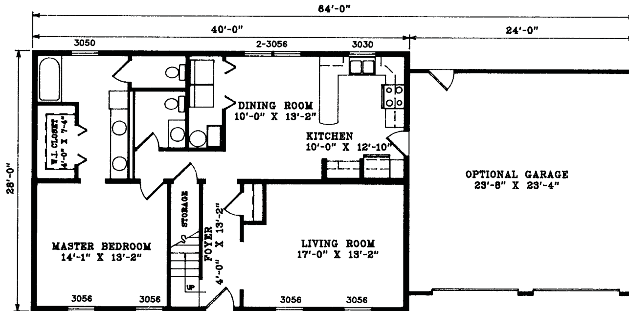
1ST STORY
