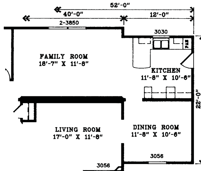
OPTIONAL 264 SQ. FT. FAMILY RM. FLOOR PLAN
