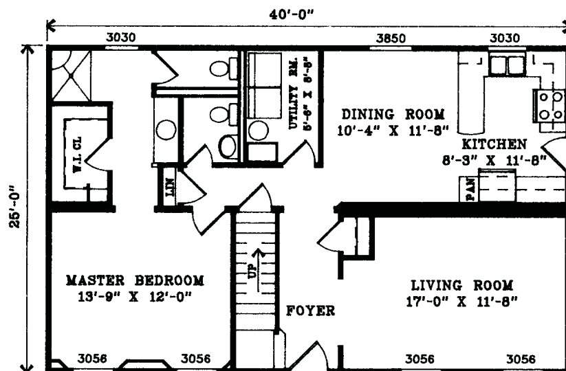
1ST STORY FLOOR PLAN
