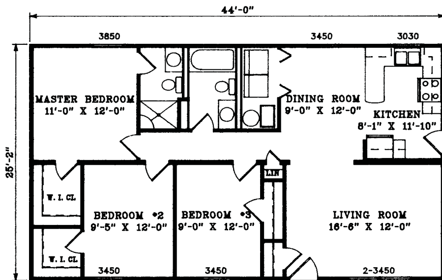
CRAWLSPACE MODEL (SIDE GARAGE ADAPTABLE)
