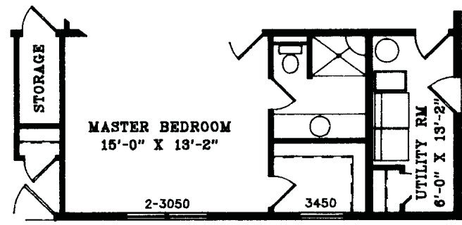
CRAWLSPACE MODEL (SIDE GARAGE ADAPTABLE)
