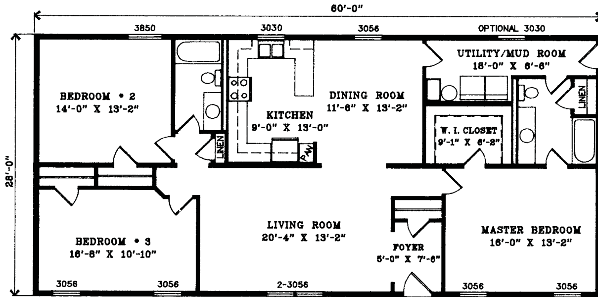
CRAWLSPACE MODEL (SIDE GARAGE ADAPTABLE)
