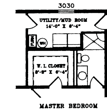
CRAWLSPACE MODEL---OPTION #1
