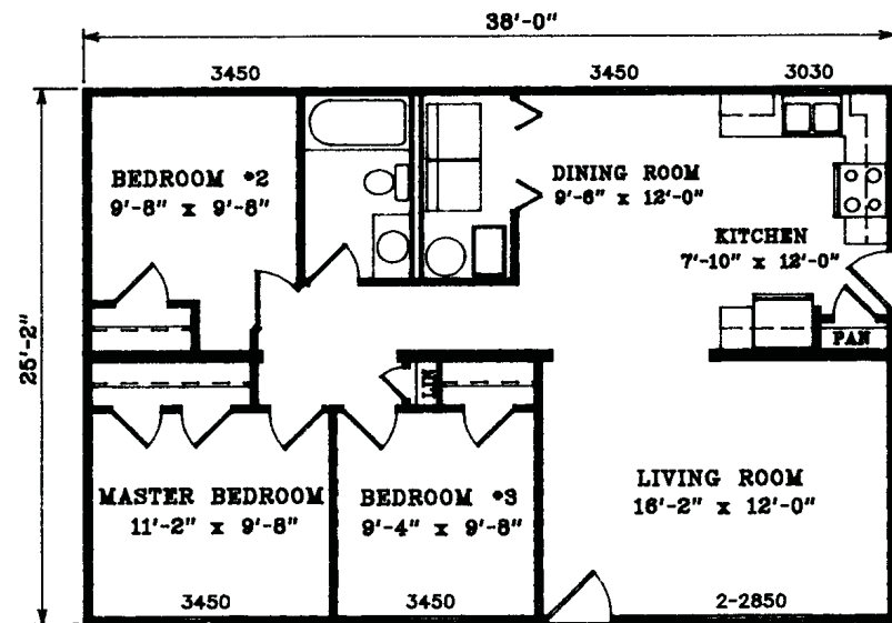
CRAWLSPACE MODEL (SIDE GARAGE ADAPTABLE)
