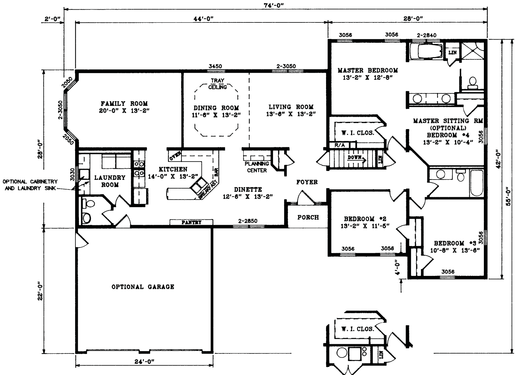
BASEMENT MODEL
