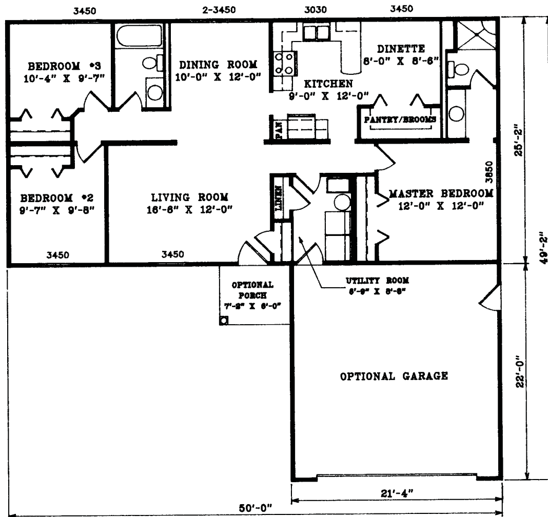
CRAWLSPACE MODEL
